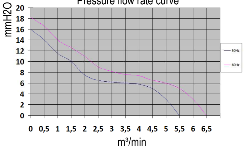
Curva pressione portata Pressure flow rate curve
